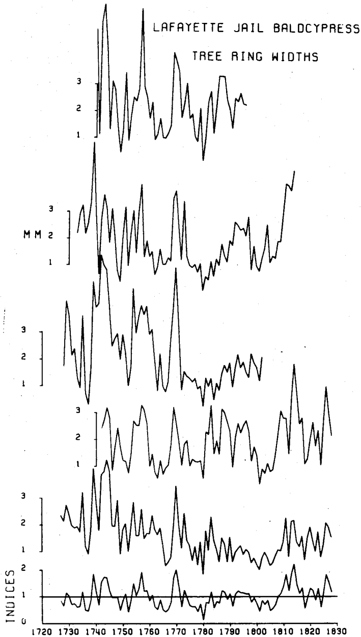
Figure 9. Crossdating among five baldcypress specimens (028311, -161, -231, -151, -041 from the top) and the mean index chronology (lower plot) from the Lafayette County Jail.
